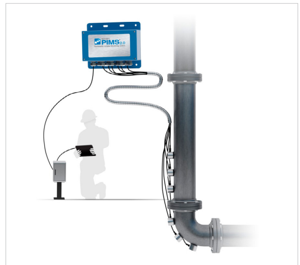
Figure 2: User connecting to smartPIMS Datalogger via DIU adapter and table/PC using dataPIMS software.
